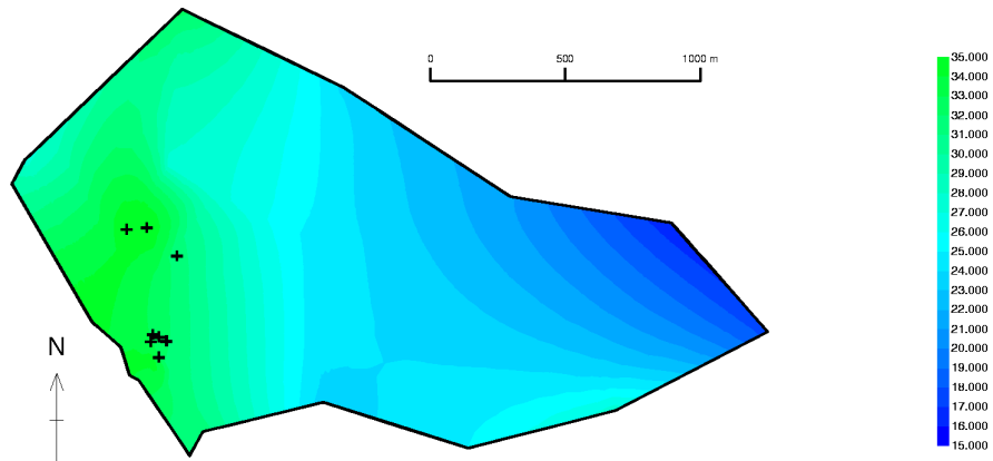
Figure 6-1 Shaded contour plot of groundwater head.
